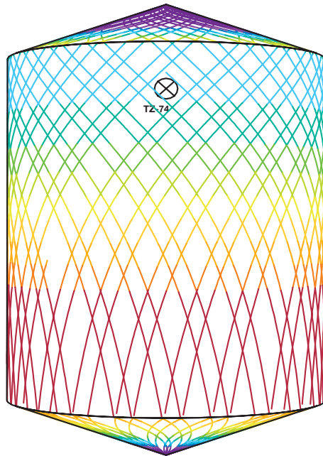
D5m H6m, Toftejorg TZ-74 Brew Kettle Version, 4 x 6 mm, 100% Time = 4.4 min., Water consumption = 907 l
