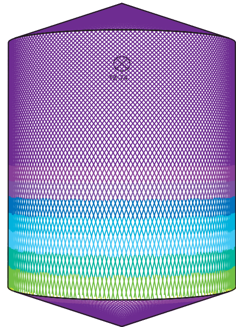
D5m H6m, Toftejorg TZ-74 Brew Kettle Version, 4 x 6 mm, 100% Time = 18.2 min., Water consumption = 3760 l
