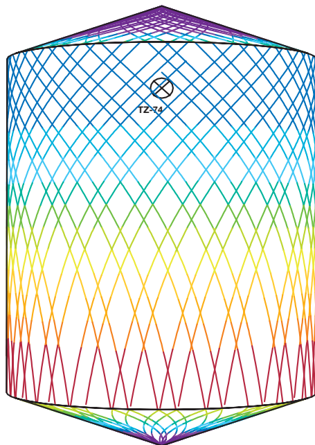
D5m H6m, Toftejorg TZ-74, 4 x 7 mm, 0% Time = 4.7 min., Water consumption = 1323 l
