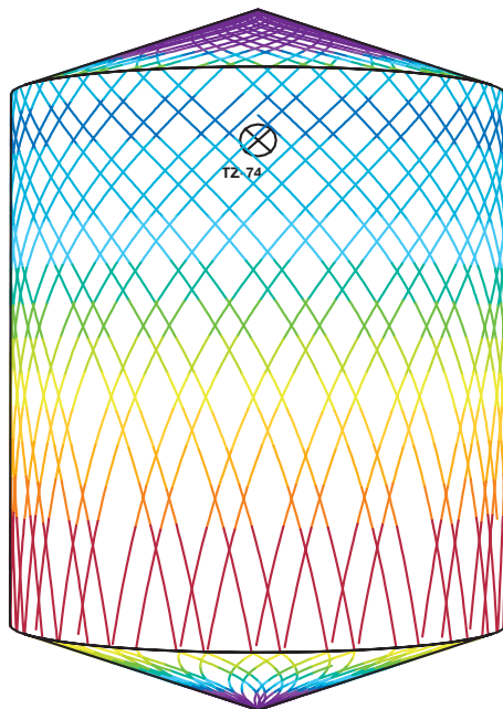
D5m H6m, Toftejorg TZ-74 Self Cleaning version, 4 x 7 mm, 0% Time = 3.8 min., Water consumption = 1192 l
